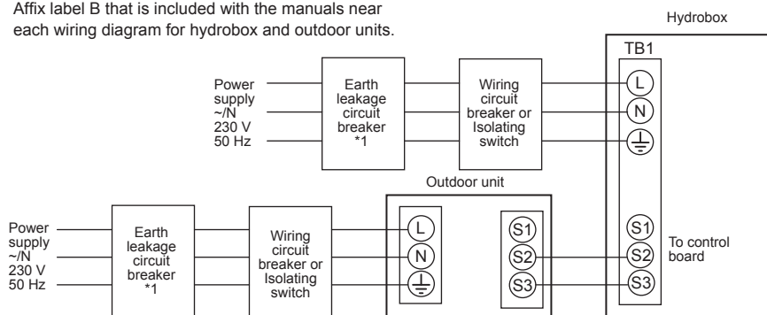
<Figure 4.4.5> Electrical connections 1 phase
