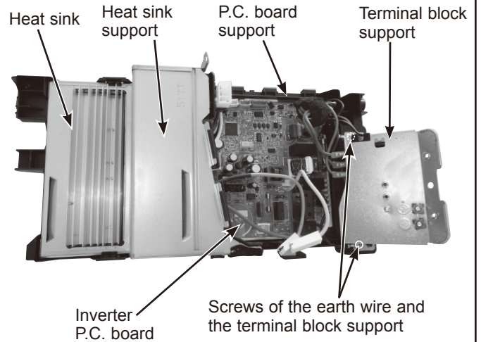
Photo 5 (Inverter assembly)
