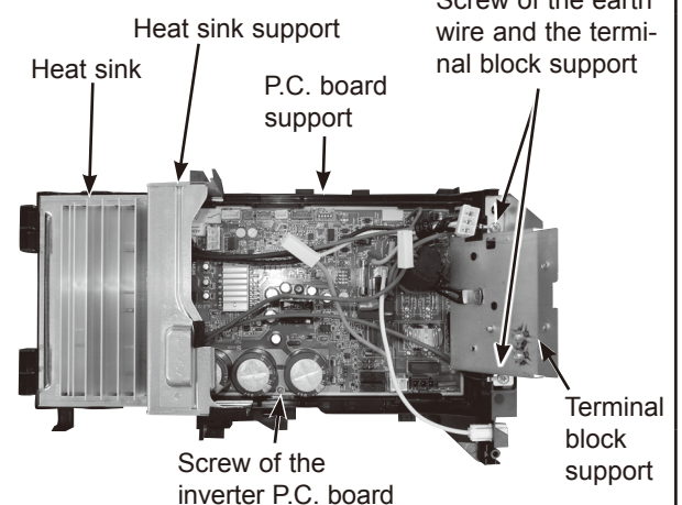
Photo 4 (Inverter assembly)
